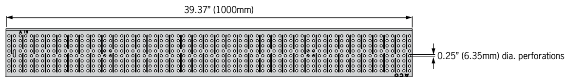
Side elevation
